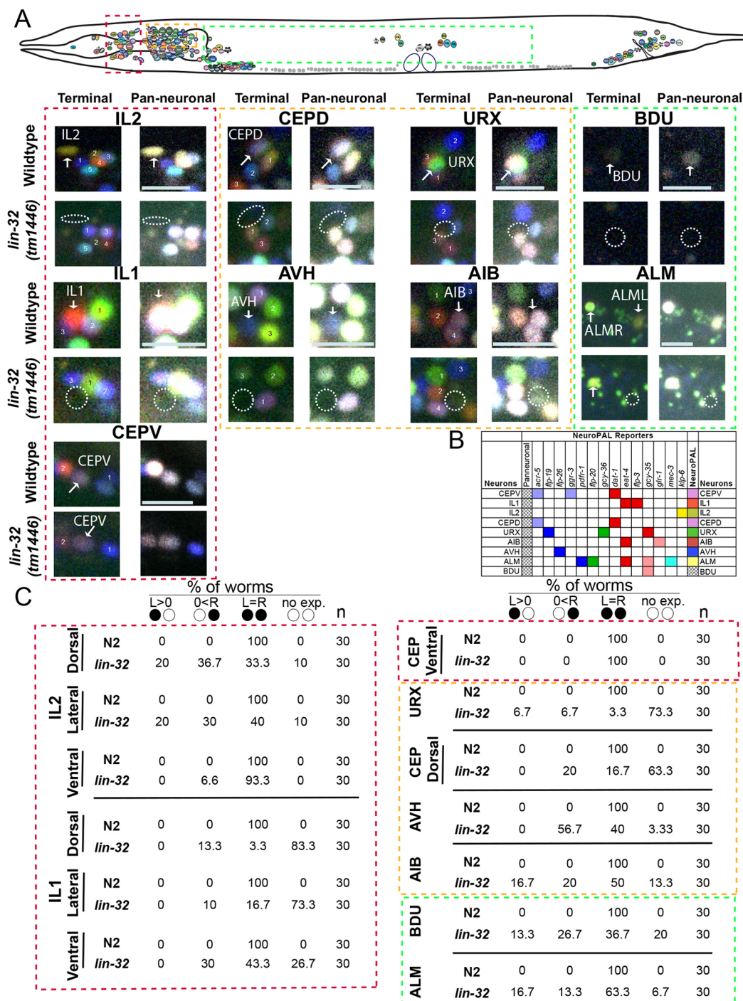
Fig. 3. Proneuronal activities of lin-32 in specific lineages. (A) The terminal, neuron type-specific and pan-neuronal identities of many neurons that express lin-32 during development are affected in lin-32(tm1446) , as revealed here using the cell-fate marker strain NeuroPAL ( otIs669 ). Boxes with different color codes highlight the ganglia for neurons (schematized at the top of the figure) exhibiting fate defects. Neurons (indicated by 1, 2, 3, etc.) that differ in wild-type versus mutant animals are indicated by arrows (see Materials and Methods for notes on cell identification); the locations where neuron colors are missing from mutants are circled by a dashed line. Neighboring neurons with similar identity in mutant and wild-type animals are labeled with corresponding numbers (some neuron colors appear to differ between wild type and mutant because some neurons lie out of the plane of focus; see Materials and Methods and Fig. S1). The neighboring neurons are used as landmarks to ID the cell of interest (see Materials and Methods). (B) The NeuroPAL reporter-fluorophore combinations that were responsible for coloring each neuron type. Cell-fate alterations are determined by changes in this color code. With this code, lost colors can be directly mapped back to losses of reporter expression, thereby determining mutant effects on cell identity. (C) Data for the terminal and pan-neuronal fate defects shown in A, indicating the percentage of animals that display the wild-type NeuroPAL color code for the indicated neuron class. No instances were observed in which the terminal markers were affected but the pan-neuronal identity remained intact. The same effects of lin-32 on dat-1 expression in CEPD (i.e. loss of expression) and CEPV (i.e. no effect detected) have been previously reported (Doitsidou et al., 2008). Circles indicate bilateral left-right homologs of the respective neuron class (L>0, expression only in left neuron; 0<R, expression only in right neuron; L=R, expression in both neurons, i.e. wild type). Scale bars: 10 \mu m.
